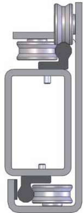
Tubular rail with external carrier for heavy loads/ moments.
