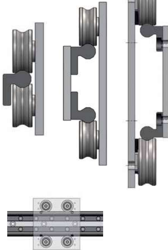
Wide rail with outer carrier
