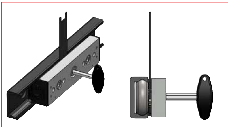
Preload setting of slider series RL.
