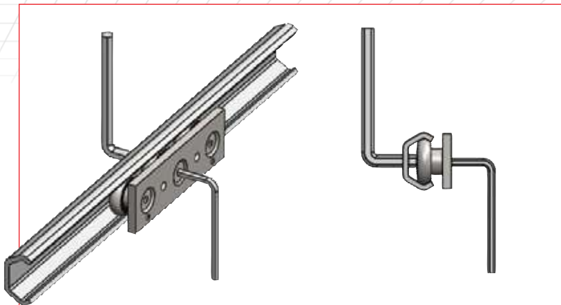
Preload setting of slider series RL.
