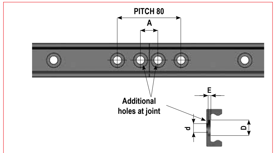
Joining area for spliced rails
