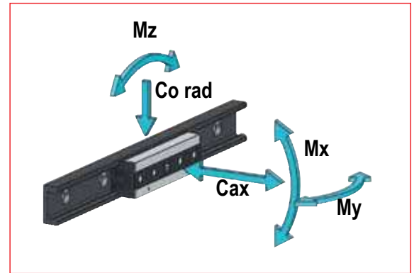
Load direction
