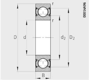
Seal 2HRS
