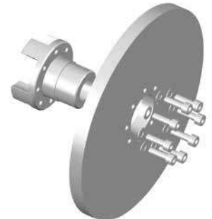
Type "GRFRD-GRFRT" execution
