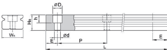
Rails MGNR
