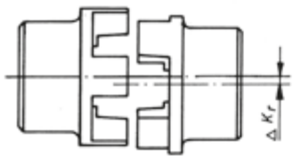
Radial misalignment
