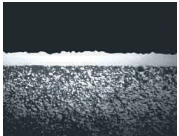
Cross-section of ATCoat coating
